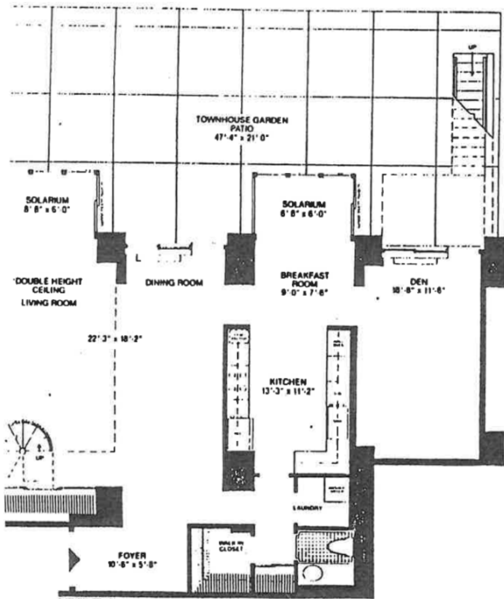
1 RIDGE Y LEVEL HOUSE UNIT #4
